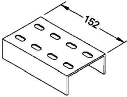
Emenda Externa "I" 38x76
