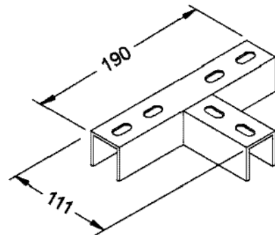
Emenda Interna "T"
