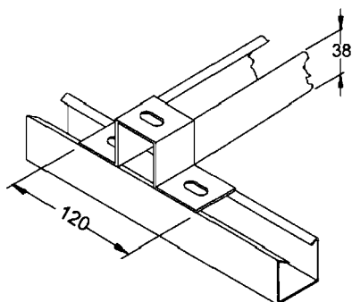
Cantoneira "ZZ"
