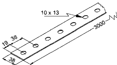
Fita Perfurada 38x3000
