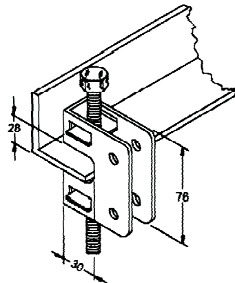
Grampo "C"
