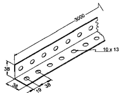
Cantoneira "L" 38x38x3000
